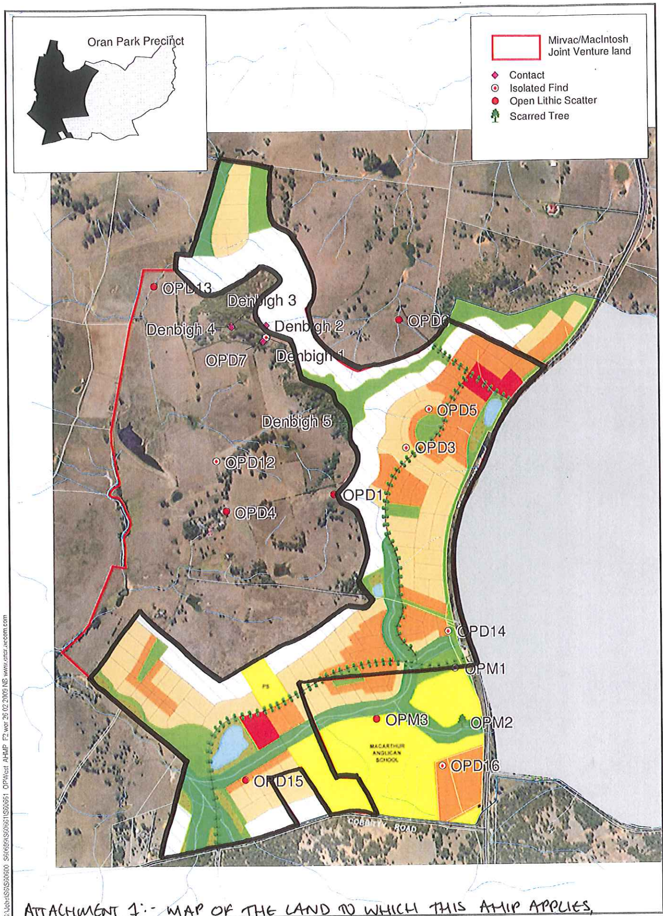
Figure F2 Interim Layout Plan
